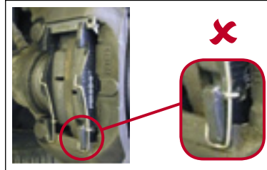
Image 2 Anti-rattle springs incorrectly located
