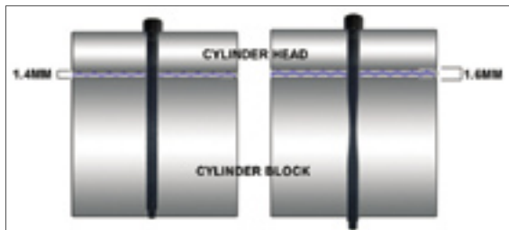
Image 1 - Cylinder head showing a new Head Bolt on the left and a stretched Head Bolt on the Right
