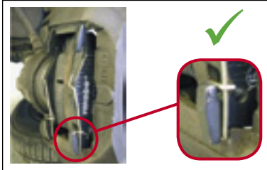
Image 1 Anti-rattle springs correctly located
